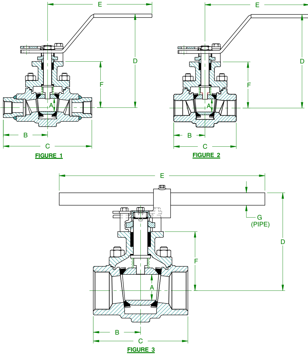
ASME CLASS 300, NPT, STANDARD PORT Dimensions in Inches
