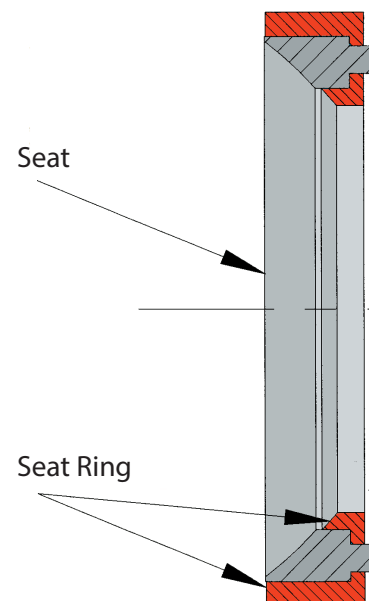
Figure 2 Seat Design 2
