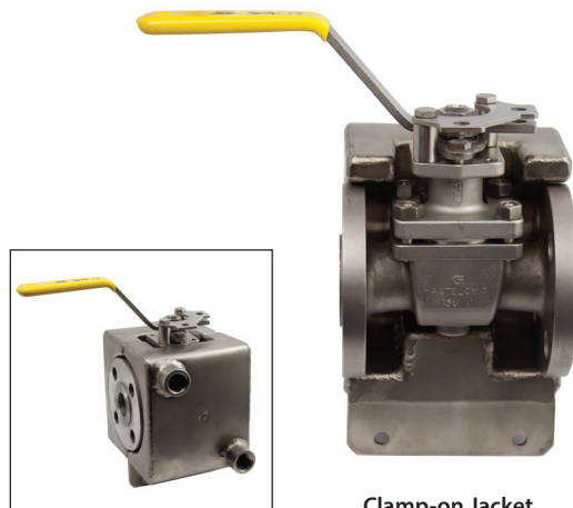
Clamp-on Jacket
