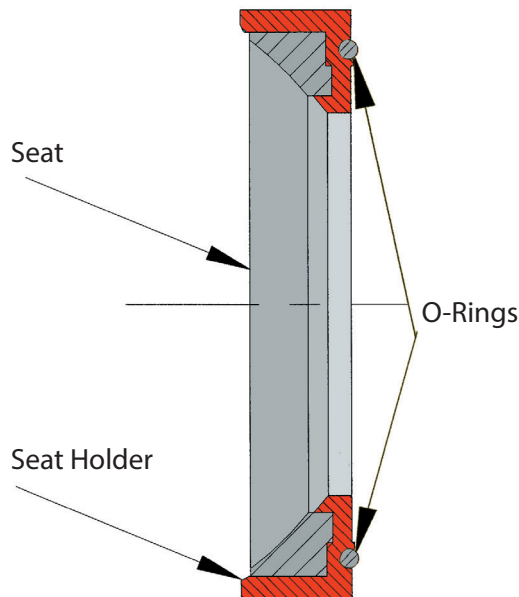
Figure 3 Seat Design 3
